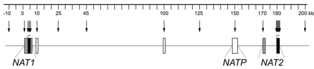
Figure 1 Schematic representation of the NATs region spanning >200 kb. Sequenced loci are represented by boxes (black boxes = coding regions; gray boxes = flanking regions; white boxes = intergenic regions), and arrows indicate the positions of genotyped SNPs.
