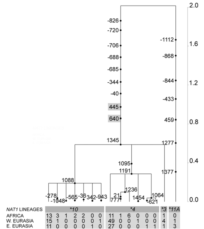
Figure 2 NAT1 gene tree. Time is scaled in millions of years. Mutations are named for their physical positions along the NAT1 locus. Lineage absolute frequencies in Africa and western and eastern Eurasia are reported. Nonsynonymous mutations are highlighted in gray.
